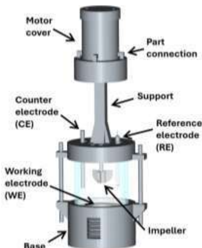
Figure 4: Electrochemical cell
