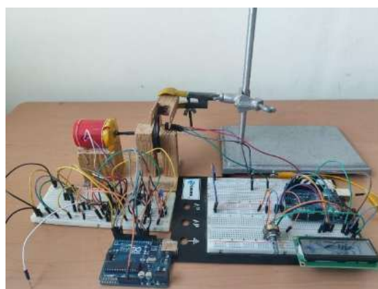
Figure 6: System on protoboard
