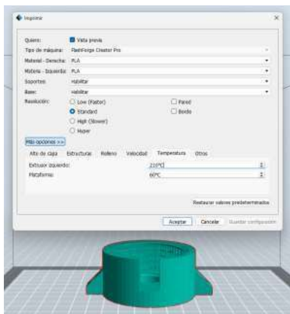
Figure 3: Printing configuration
