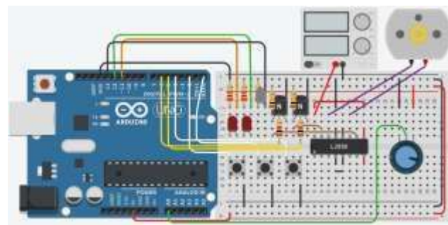
Figure 5: System simulation
