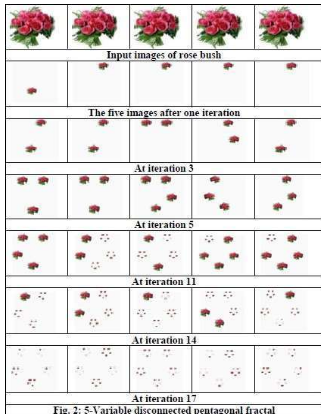
Fig. 2: 5-Variable disconnected pentagonal fractal
