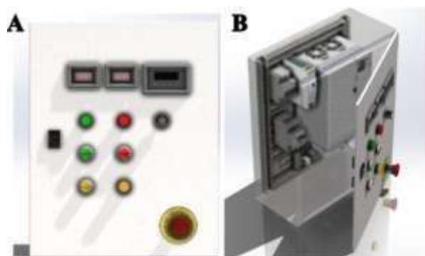
Figure 3. Design of the control and monitoring dashboard. Source: Authors.
