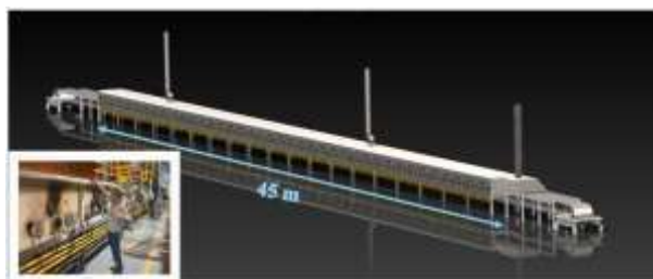
Figure 2. Schematic diagram of the production line oven. The inset shows a section of the oven. Source: Authors.
