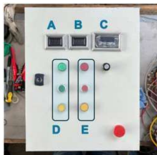
Figure 5. Final control panel. A) Inlet temperature, B) Outlet temperature, C) Belt speed, D), and E) Start, stop, and alarm reset buttons. Source: Authors.
