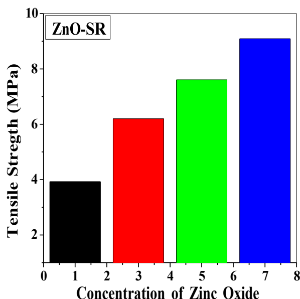
Figure 4.2 Variation of tensile strength with ZnO concentration in silicone elastomer nanocomposites.
