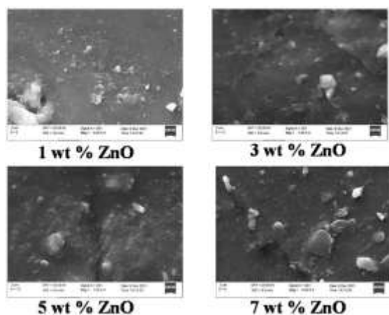
Figure 1 SEM microscopy images of ZnO/SR nanocomposites with varying nanoparticle concentrations: (a) 1%, (b) 3%, (c) 5%, and (d) 7%.
