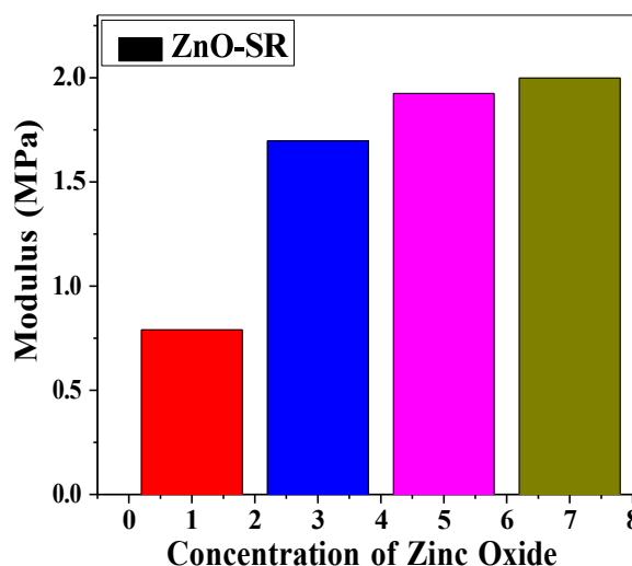
Figure 4.4 Variation of modulus with ZnO concentration in silicone elastomer nanocomposites.
