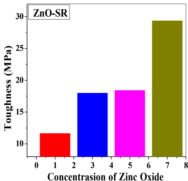
Figure 4.5 Variation of toughness with ZnO concentration in silicone elastomer nanocomposites
