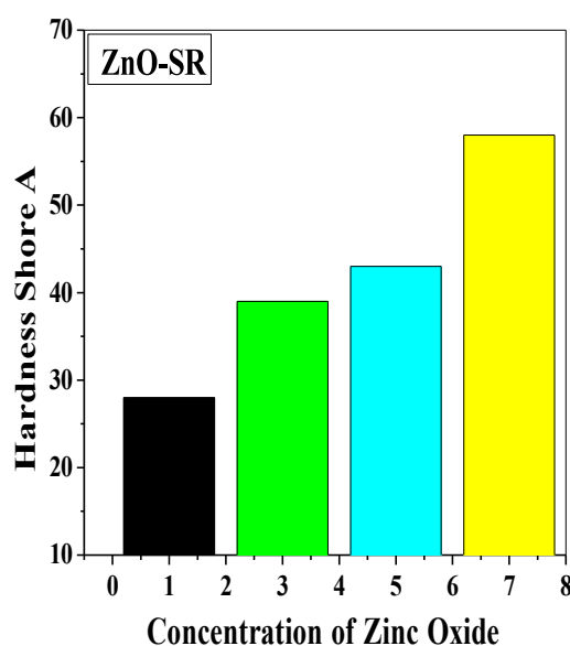
Figure 4.1 Variation of hardness with Zinc oxide
