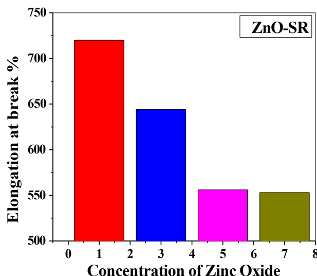
Figure 4.3 Variation of elongation at break with ZnO concentration in silicone elastomer nanocomposites.
