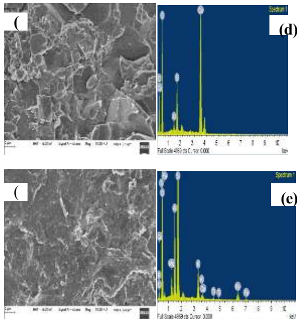
Fig. 9 SEM micrographs and EDS analysis for all 5 types of samples
