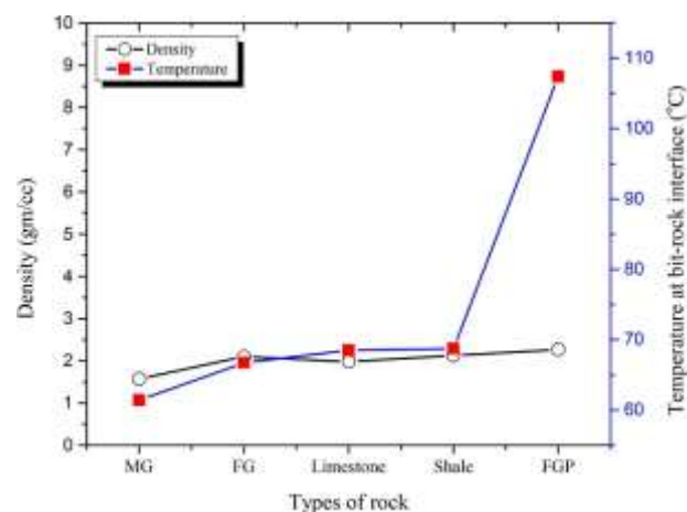
Fig. 8 Effect of interface temperature on density
