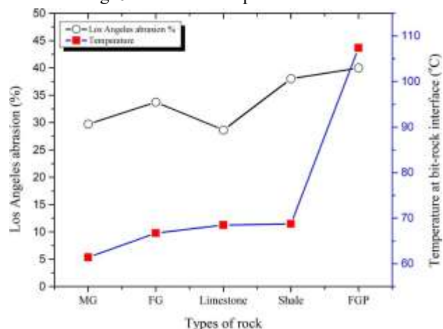
Fig. 7 Effect of temperature on Los Angeles abrasion loss
