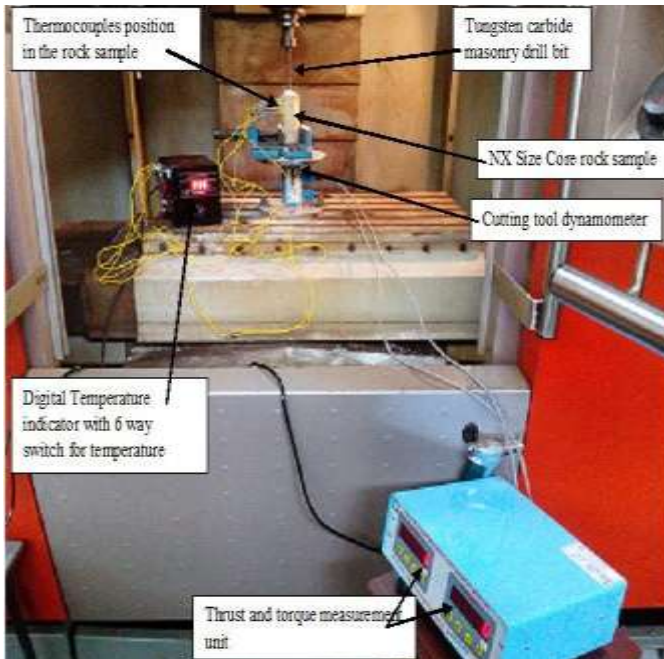
Fig. 1 A detailed setup for measuring rotary drilling temperature at the bit-rock interaction.
