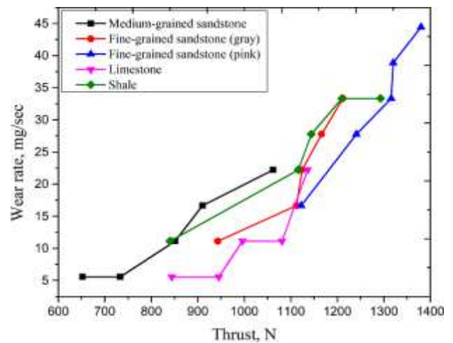
Fig. 11 Interaction between wear and thrust for different rock samples
