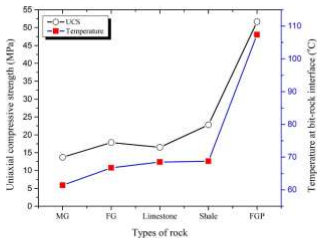
Fig. 5 Effect of temperature on UCS.
