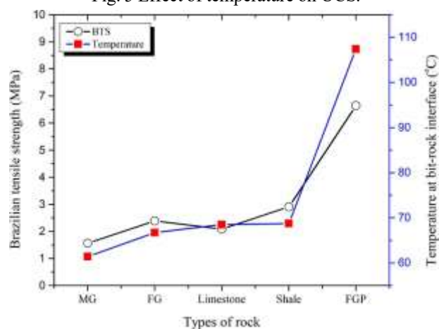
Fig. 6 Effect of at temperature on BTS
