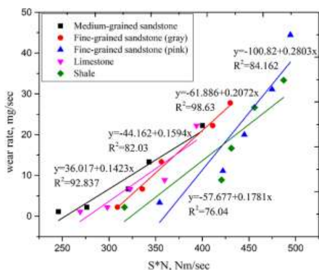
Fig. 13 Function of Spindle speed and load on wear rate
