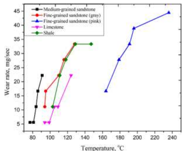
Fig. 12 Impact of temperature on drill bit wear rate.
