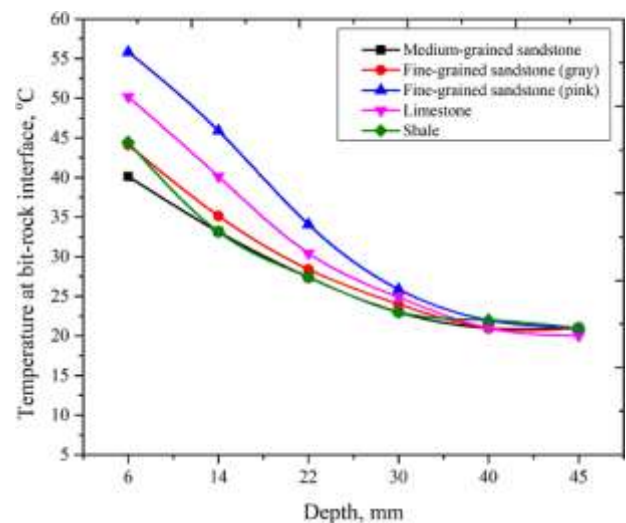
Fig. 4 Variation of temperature in the rock samples.
