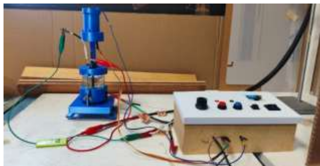
Figure 7: System assembly for testing
