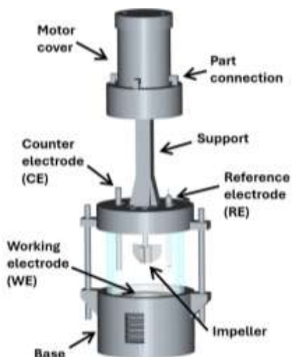
Figure 4: Electrochemical cell
